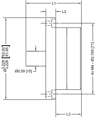
Rear Power Non-Contact Transmitter
