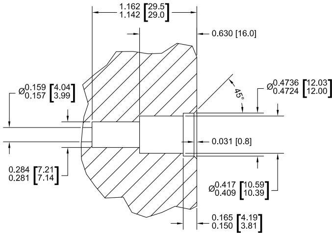
Mounting requirements for SB-3210
