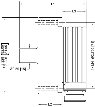
Rear Power Slip Ring Transmitter
