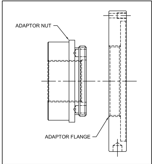
Two Part Adaptor Types 3,4,5,6
